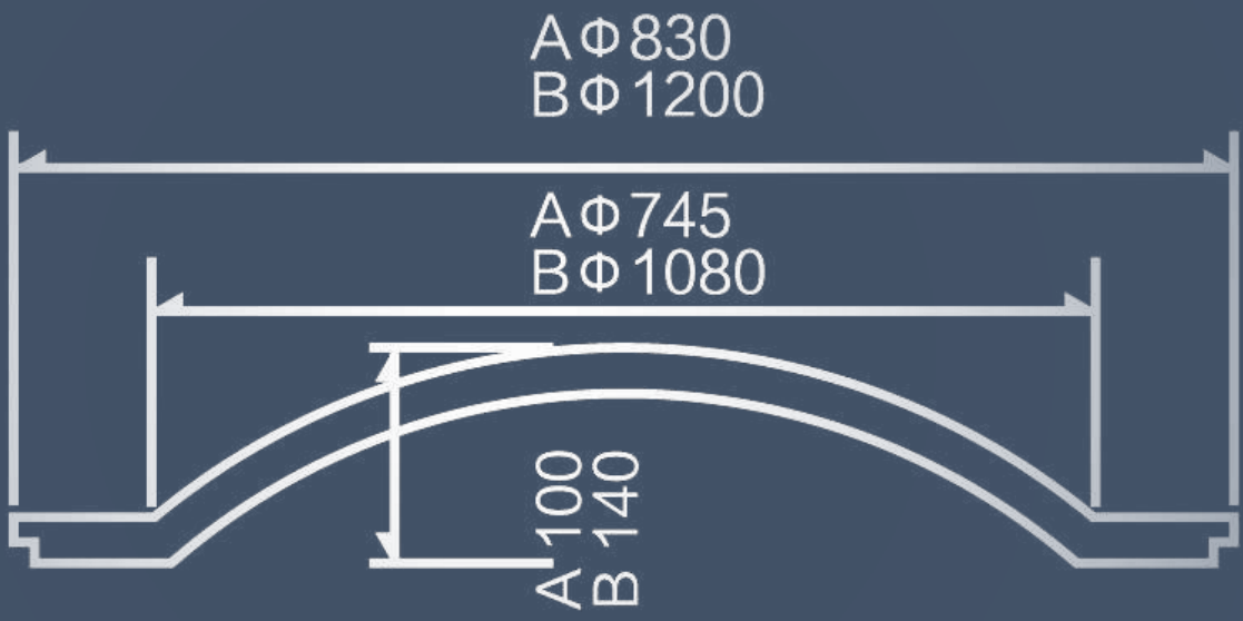
D501 A / D501 B DIAMETER — 830mm / 1200mm
